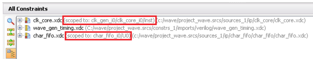
Figure 2-42: Timing Constraints All Constraints List (Example Two)
