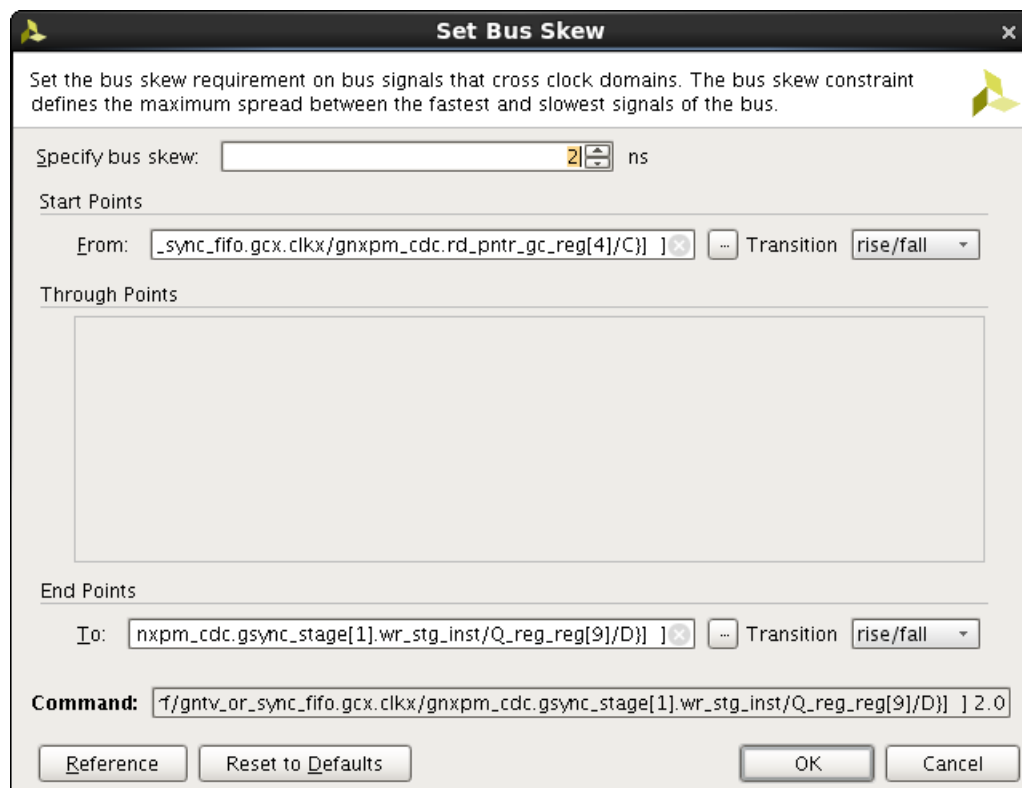
Figure 6-2: Set Bus Skew Dialog Box
