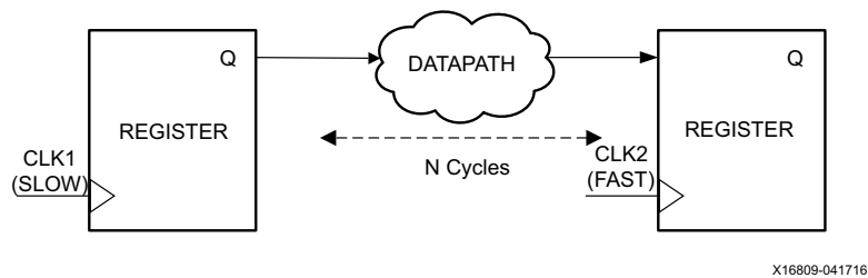
Figure 5-15: Multicycles Between SLOW-to-FAST Clocks
