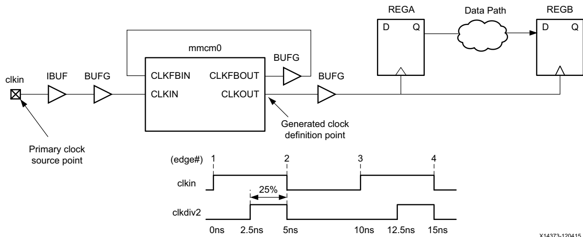
Figure 3-5: Generated Clock Example Three
