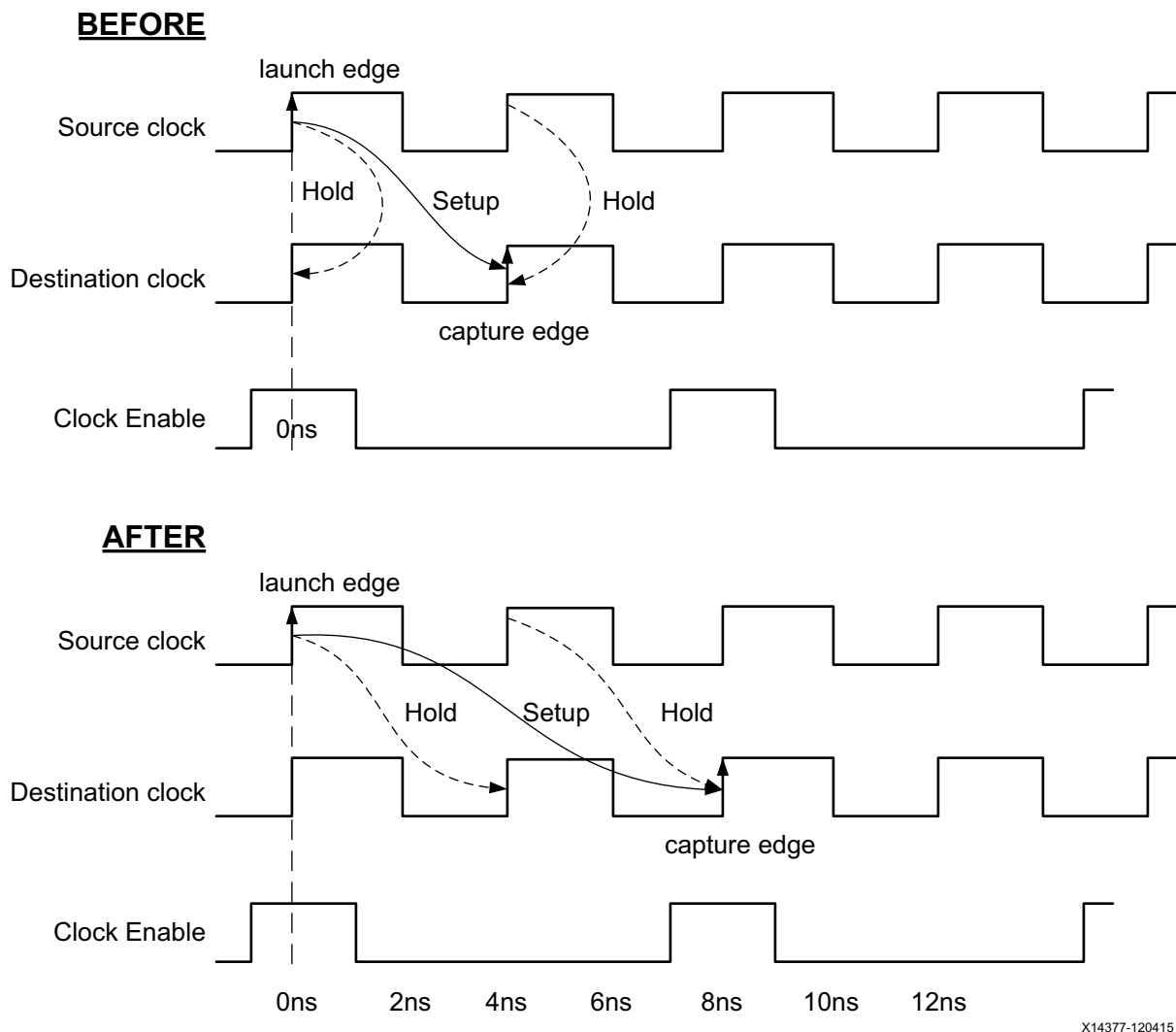
Figure 5-5: MultiCycle Path: Relaxing Setup Only
