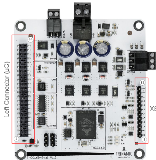
Figure 4: TMCC160-EVAL connectors
