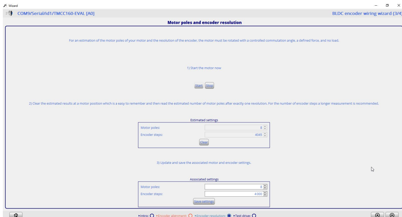
Figure 12: Encoder Wizard - 编码器分辨率
