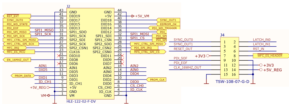
Figure 3: TMC8462-EVAL: Left connector 和 J4
