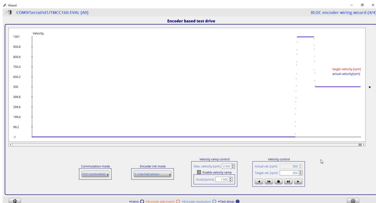
Figure 13: Encoder Wizard - Test drive
