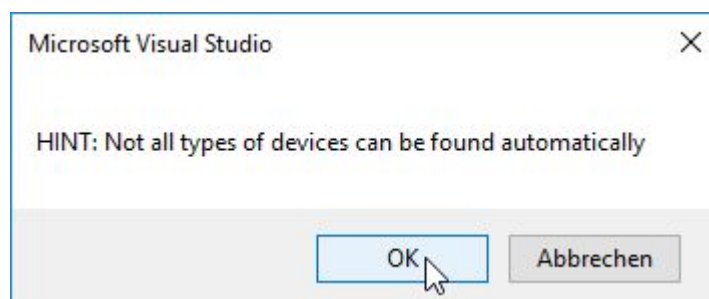
Figure 17: Confirm
