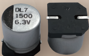
SMD
